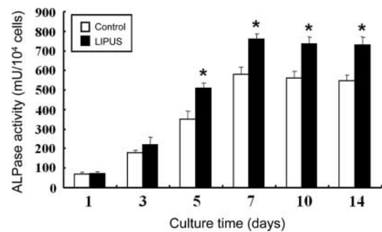
Fig. 3 Effect of LIPUS stimulation on ALPase activity The cells were cultured in the presence and absence of daily LIPUS stimulation and ALPase activity were determined at Days 1, 3, 5, 7, 10, and 14 of culture. The data are shown as the mean \pm SD of three separate experiments. * P < 0.05 for LIPUS-treated versus control
