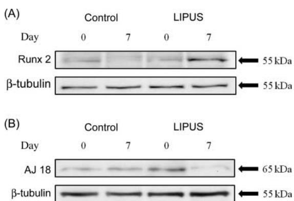
Fig. 5 Effect of LIPUS stimulation on expression levels of osteogenesis-related proteins The protein expression of Runx2 (A) and (B) AJ18 in ROS cells was determined by western blotting analysis of cells cultured at Day 7 in the presence and absence of daily LIPUS stimulation. The protein expression of BSP (C) in ROS cells was determined by western blotting analysis of cells cultured at Day 14 in the presence and absence of daily LIPUS stimulation
