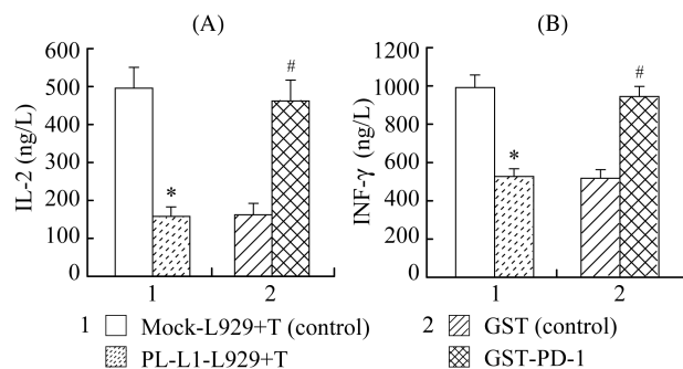
Fig. 4 Bioassays of GST-PD-1 fusion protein
