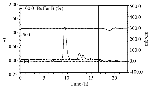
Fig. 3 Purification of GST-PD-1 by size exclusion column
